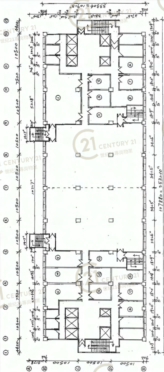
Kwai Shun Industrial Building 5 th Floor Plan 葵順工業大廈 5 樓平面圖
