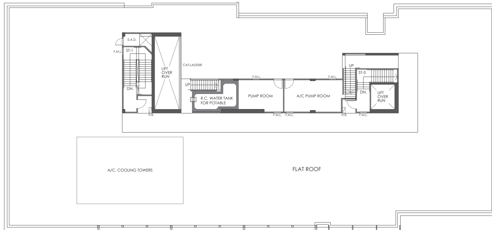
UPPER ROOF PLAN
