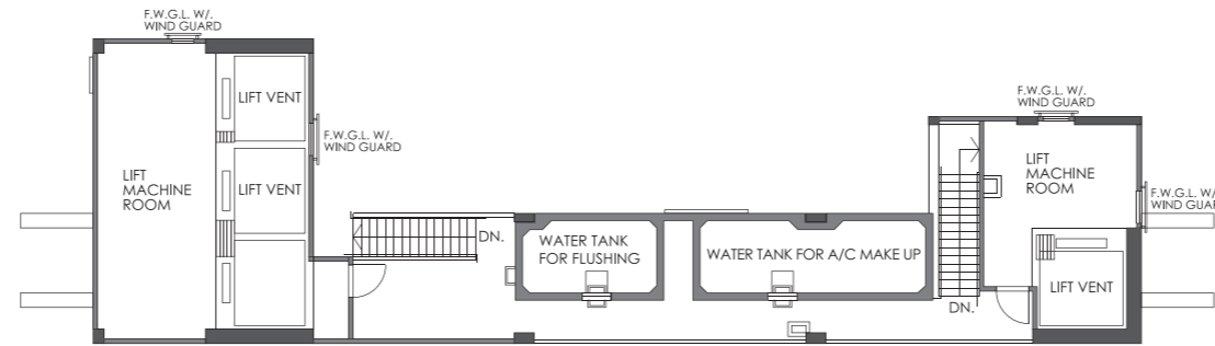
UPPER ROOF PLAN
