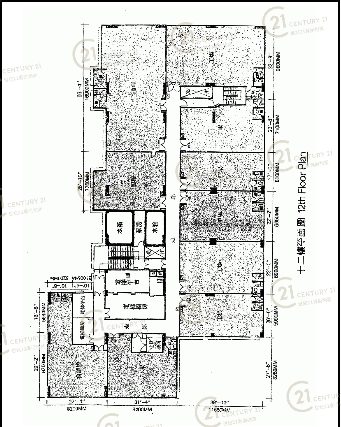
金發工業大廈1期 Kingsford Industrial Building Phase 1
