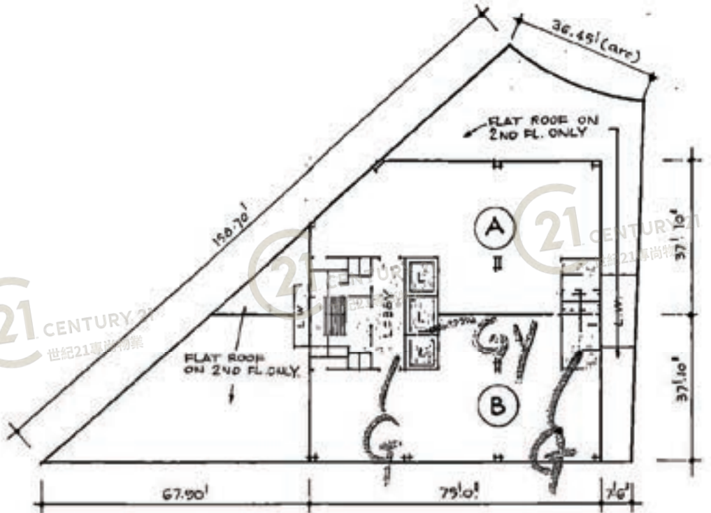
2ND. TO 21ST. FL. PLAN
