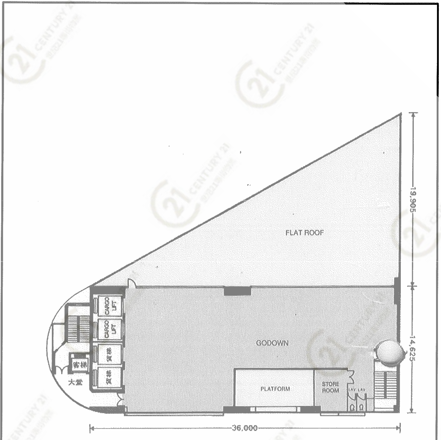
3RD FLOOR PLAN 三樓
